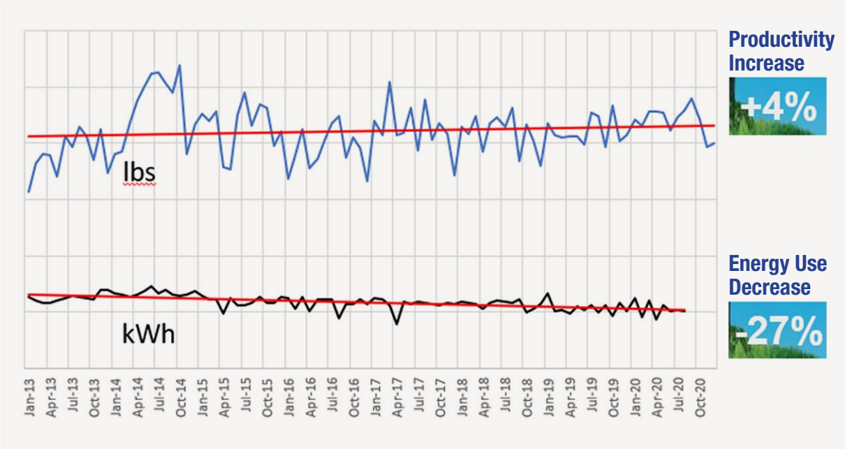
Bead mill where productivity has been increased at the same time energy use has decreased.
